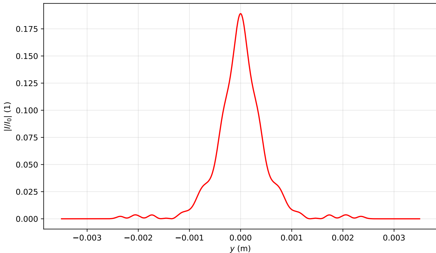
Intensity profile I(x=0, y, z=2.707)/I_0 , \text{Pin}=5.0\text{Pcr} , artificial time
